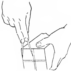
FIG. 285. CENTERING STOCK.
